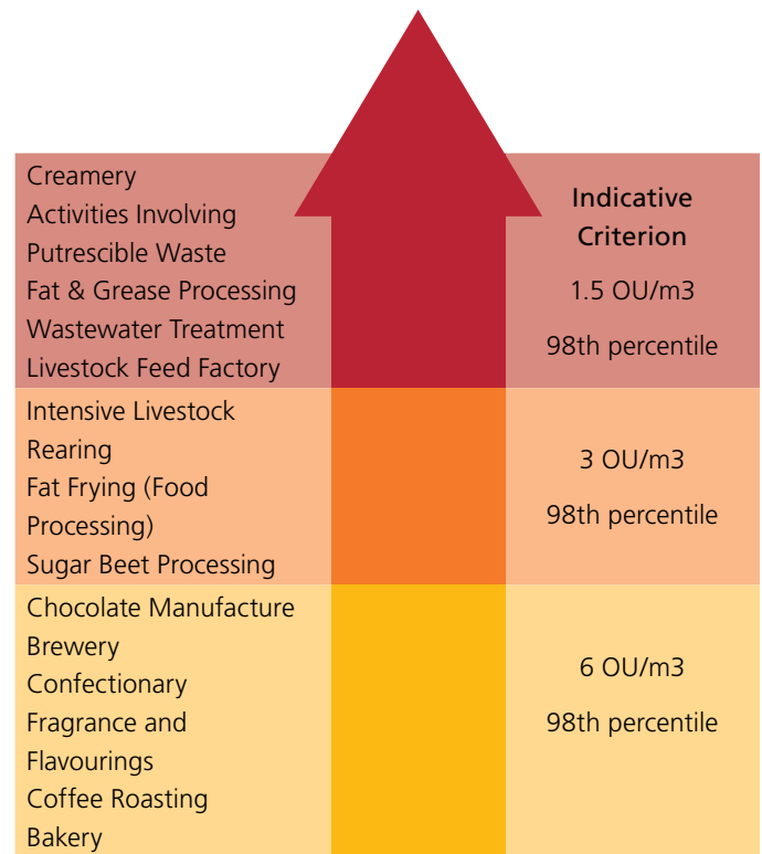
Figure 2: Indicative odour exposure criteria for ground level concentration of mixtures of odorants, from Environment Agency (2002a)
