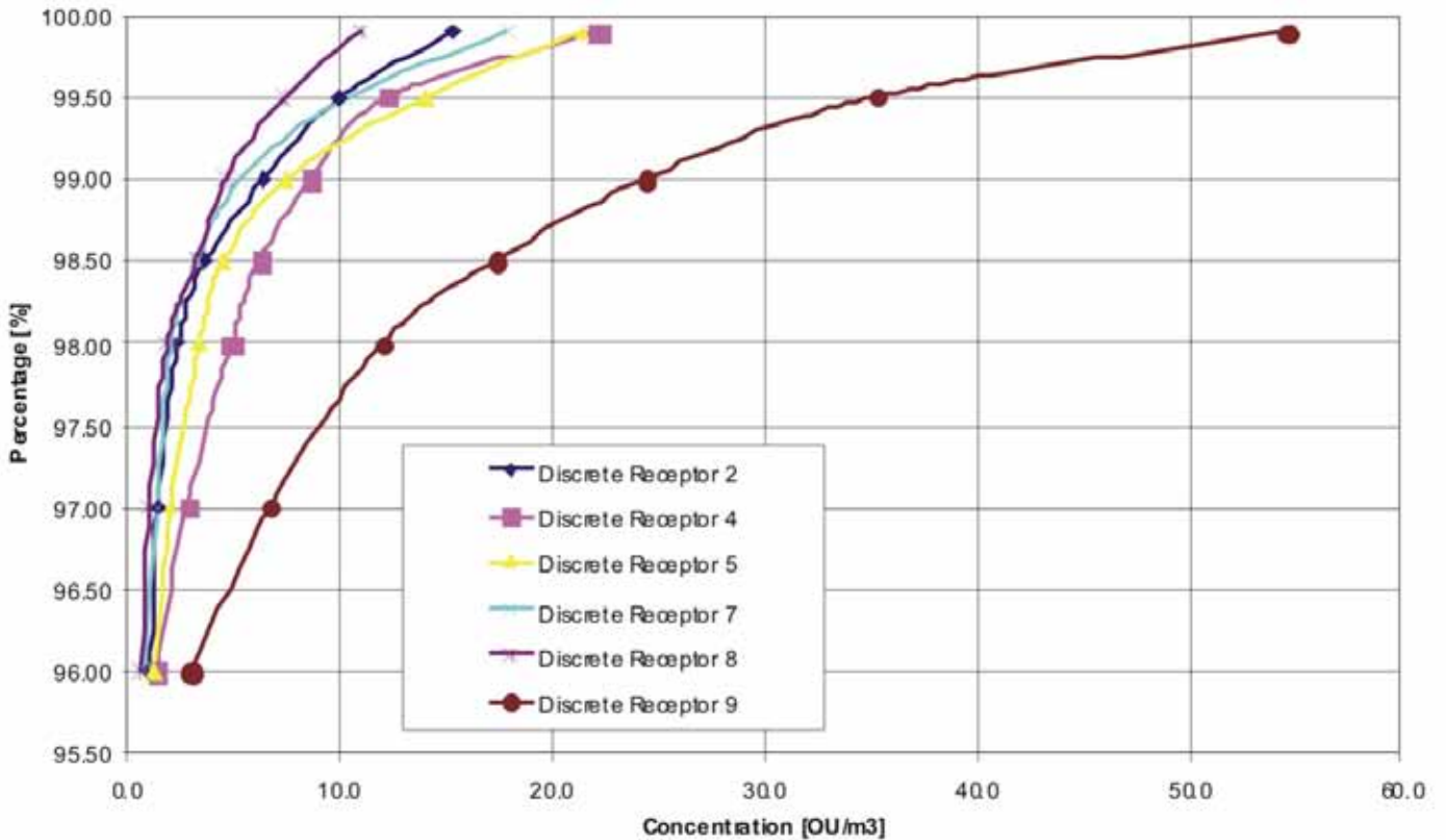
Figure 3: Ground-level concentrations for odour dispersion from brewhouse kettle stack for various percentile factors
